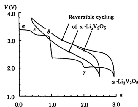
Fig. 2 Various phases associated with the electrochemical intercalation of lithium into \text{V}_2\text{O}_5 . 40
