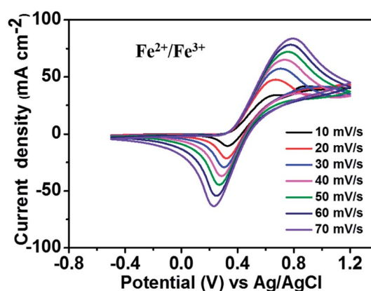
Fig. 2 CV curves of 1.5 M \text{FeCl}_2 in a 3 M HCl using GC electrode at various scan rates.
