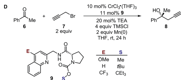
Fig. 2 (A) Desymmetrization of bisphenol. (B) Charton–LFER model. (C) Sterimol–LFER model. (D) Nozaki–Hiyama–Kishi propargylation of acetophenone.
