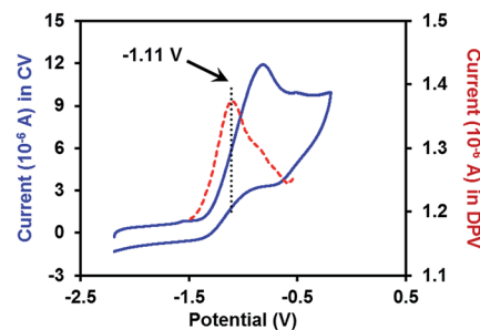
Fig. 2 CV and DPV plots of 2 mM complex 4 ·DME in THF (0.1 M n-Bu_4N^+PF_6^- as the supporting electrolyte). The blue solid line: CV plot (scan rate = 0.1 V s^{-1} ); the red dashed line: DPV plot.
