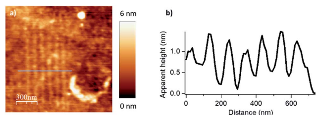
Fig. 4 Resolution limit, for the esterification reaction with myristic anhydride as acylating reagent, with F = 2900 \text{ nN} , V_{scan} = 2 \mu m s^{-1} . (a) Topography image in tapping mode of an array of covalently attached nanostructures by catalytic local acyl transfer. (b) Line profile (corresponding to the blue line in (a)) displaying a lateral resolution down to 45 \pm 5 nm (FWHM).
