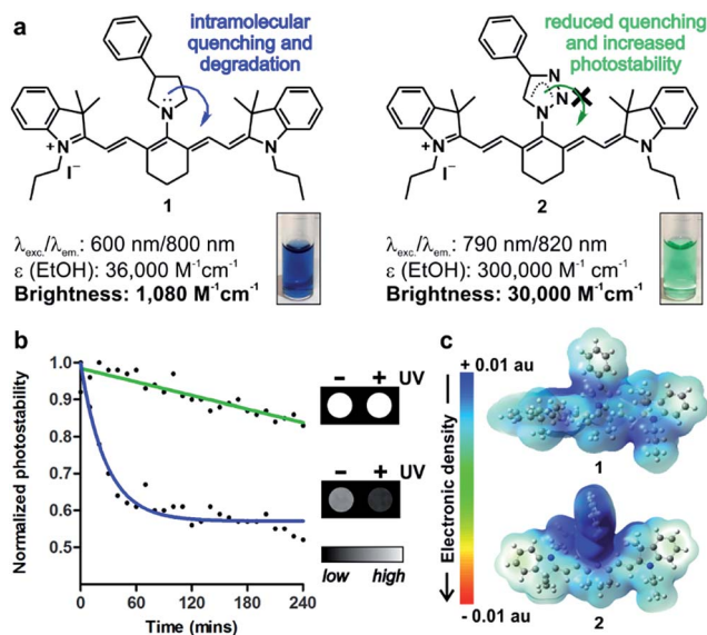
Fig. 1 (a) Chemical structures and properties of isosteric tricarbo-cyanine N -amines (1) and N -triazoles (2) in EtOH. (Inset) Absorbance pictograms of compounds 1 and 2 (10 \mu M). (b) Photostability analysis of compounds 1 (blue) and 2 (green) (both at 50 \mu M in PBS) under continuous light irradiation. Solid lines correspond to one phase exponential decay regressions for both sets of values. (Inset) NIR fluorescence pictograms of compounds 1 and 2 (10 \mu M in PBS) before and after UV light irradiation. (c) Pseudo-coloured electronic distribution maps for compounds 1 (top) and 2 (bottom) in their fundamental state.
