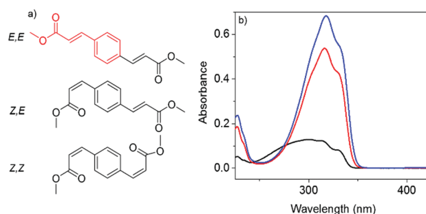
Fig. 1 (a) The three geometric isomers for DPD, with the methyl cinnamate base unit highlighted in red. (b) Steady-state absorption spectra for E,E -DPD: at ~10 μM concentration in ethanol (blue line) and acetonitrile (red line), and (owing to poorer solubility) <10 μM for E,E -DPD in cyclohexane (black).
