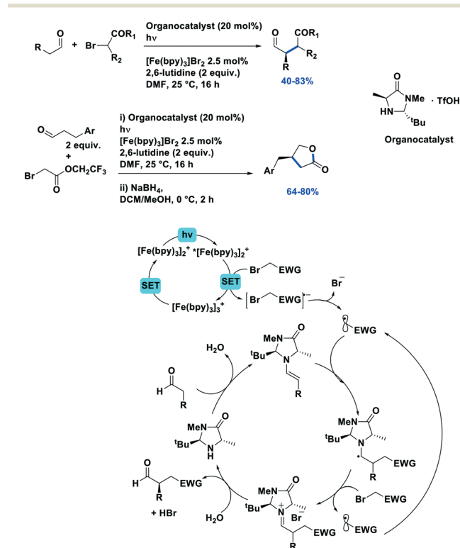
Fig. 47 a) Scope of the stereoselective alkylation promoted by [\text{Fe}(\text{bpy})_3]\text{Br}_2 ; b) preparation of enantioenriched lactones via alkylation of aldehydes.
