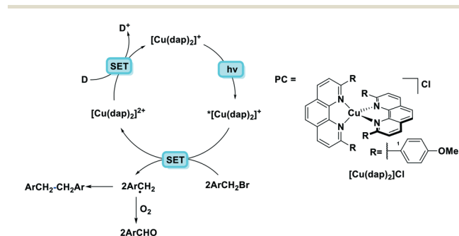
Fig. 12 Photoredox catalyzed reaction using a copper(i) complex reported by Sauvage et al. D represents an electron donor such as alkyl amines. 46
