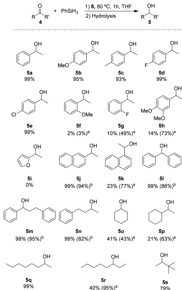
Scheme 2 Substrate screening for the hydrosilylation of ketones catalysed by 8. Reaction conditions: 0.5 mmol substrate, 0.25 mol% of 8, 1 mmol of silane, 0.2 mL THF, 80 °C, 1 h. Quantified by 1 H NMR using mesitylene or tetradecane (0.5 mmol) as the internal standard. a 1 mol% catalyst loading. b Isolated yield.
