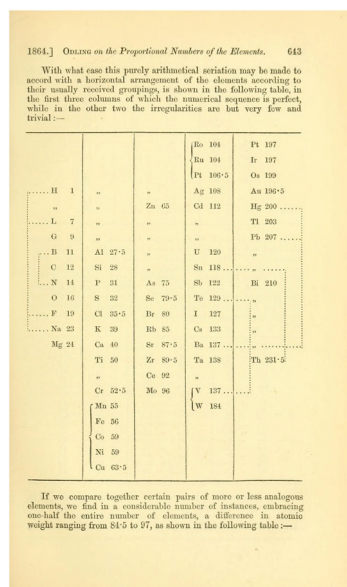
Fig. 6 The table from Odling showing the periodic behaviour within each (horizontal) group (retrieved from https://www.biodiversitylibrary.org/item/52516#page/675/mode/1up ). 53
