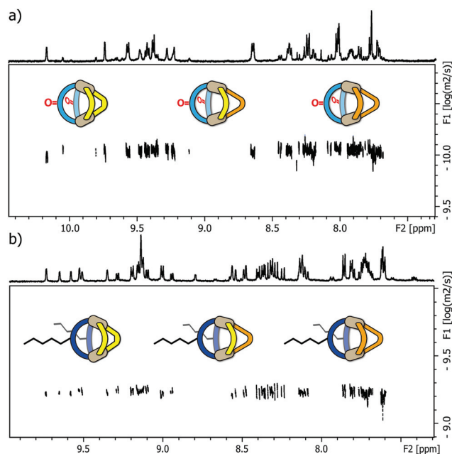
Fig. 3 (a) ^1\text{H} DOSY NMR spectrum of a mixture of heteroleptic cages [\text{Pd}_2\text{L}^{\text{F}}_2\text{L}^{\text{P}}_1\text{L}^{\text{P}'}_2]^{4+} , [\text{Pd}_2\text{L}^{\text{F}}_2\text{L}^{\text{P}}_1\text{L}^{\text{P}'}_1]^{4+} and [\text{Pd}_2\text{L}^{\text{F}}_2\text{L}^{\text{P}}_2\text{L}^{\text{P}'}_2]^{4+} (depicted from left to right, 500 MHz, 298 K, \text{DMSO}-d_6 ); (b) ^1\text{H} DOSY NMR spectrum of a mixture of heteroleptic cages [\text{Pd}_2\text{L}^{\text{C}}_2\text{L}^{\text{P}}_2]^{4+} , [\text{Pd}_2\text{L}^{\text{C}}_2\text{L}^{\text{P}}_1\text{L}^{\text{P}'}_1]^{4+} and [\text{Pd}_2\text{L}^{\text{C}}_2\text{L}^{\text{P}}_2]^{4+} (depicted from left to right, 500 MHz, 298 K, \text{CD}_3\text{CN} ). In both cases, the depicted DOSY spectra do not allow a clear discrimination of the different species.
