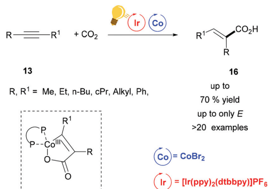
Scheme 7 Alkyne Carboxylation via synergistic Ir(III)-photoredox/Co catalysis. Reagents and conditions: alkyne 13 (1.00 equiv.), CO 2 (1 atm), Ir-photocat. (1 mol%), CoBr 2 (10 mol%), dcyt (10 mol%), ZnBr 2 (1 equiv.), i-Pr 2 NEt (3.00 equiv.), in CH 3 CN, blue LED, 24 h. 51
