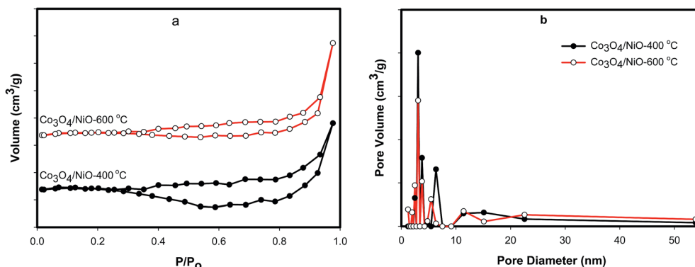
Fig. 6 \text{Co}_3\text{O}_4/\text{NiO} microspheres: (a) N_2 sorption isotherms; (b) micro- and mesopores distributions.
