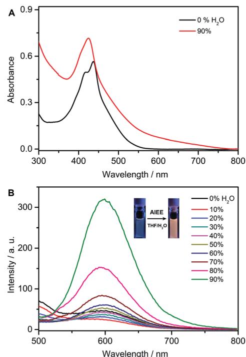
Fig. 4 AIEE behavior of the copolymer P(NIPAM-co-EM) (15.6 μM) in H 2 O/THF mixtures with different f_w . \lambda_{ex} = 430 nm; inset (B): fluorescence images of the P(NIPAM-co-EM) ( f_w = 0 and 90%) under UV light irradiation.
