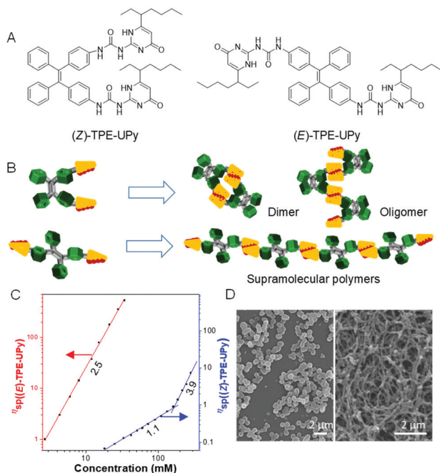
Fig. 9 (A) Structure of ( Z )-TPE-UPy and ( E )-TPE-UPy. (B) Schematic presentation of supramolecular polymerization of ( Z )- and ( E )-TPE-UPy in chloroform at 298 K on the solution viscosity with best-fit lines and slopes. (D) SEM images of particles of ( Z )-TPE-UPy (left) and nanofibers of ( E )-TPE-UPy (right). Reproduced from ref. 70 with permission from ACS Publications.
