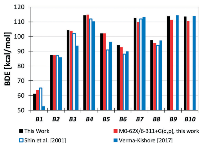
Fig. 3 BDEs of vanillin [kcal mol −1 ]. Comparison of literature 48,50 and predicted values.
