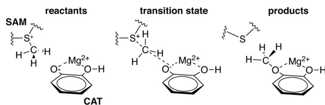
Scheme 1 Reaction for COMT-catalyzed methylation of CAT substrate by SAM.
