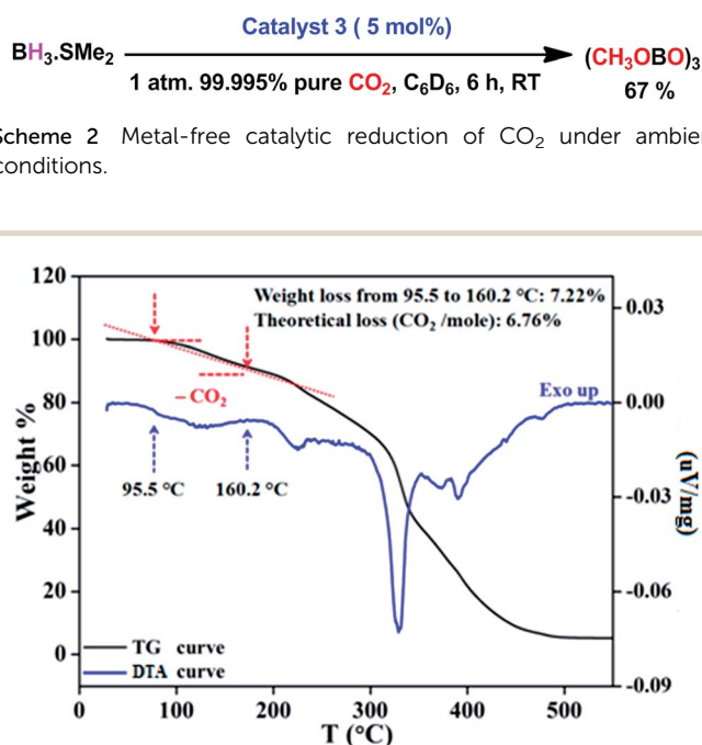
Fig. 3 Removal of captured \text{CO}_2 in solid state, as monitored by thermogravimetric-differential thermal analysis of compound 3 .
