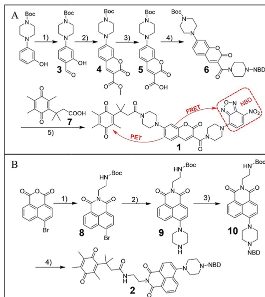
Fig. 1 (A) Synthesis route for probe 1. (1) POCl 3 , DMF, rt, 34%; (2) dimethyl malonate, piperidine, rt, 84%; (3) THF/10% NaOH = 1 : 1, rt, then 1 M HCl, 70%; (4) NBD-PZ, EDCI, DMAP, rt, 67%; (5) DCM/TFA = 1/1, then Q 3 PA, EDCI, DMAP, rt, 44%. (B) Synthesis route for probe 2. (1) N -Boc-ethylenediamine, reflux, 65%; (2) piperazine, reflux, 63%; (3) NBD-Cl, TEA, rt, 66%; (4) DCM/TFA = 1/1, then Q 3 PA, EDCI, DMAP, rt, 88%.
