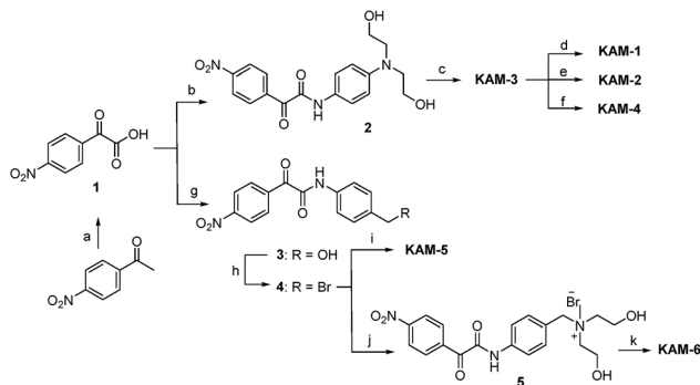
Scheme 2 Synthesis of KAM prodrugs. Reactants and conditions: (a) \text{SeO}_2 , pyridine, 90 °C, \text{N}_2 , 35%; (b) N -4-aminophenyl diethanolamine, EDCI, DIEA, DMF, 42%; (c) \text{MeSO}_3\text{Cl} , DMAP, TEA, DCM, reflux, 70%; (d) \text{LiCl} (5 eq.), DMF, 60 °C, 65%; (e) \text{NaBr} (5 eq.), DMF, 60 °C, 67%; (f) \text{LiCl} (1 eq.), MeCN, 60 °C, 23%; (g) (4-aminophenyl)methanol, EDCI, DIEA, DMF, 33%; (h) \text{CBr}_4 , \text{PPh}_3 , DCM, 0 °C–r.t., 50%; (i) N -(4- N , N' -dime-thylaminophenyl)-bis(2-chloroethyl)amine, MeCN, 43%; (j) N -methyl-diethanolamine, \text{CHCl}_3 , reflux, 76%; (k) \text{SOCl}_2 , r.t., 62%.
