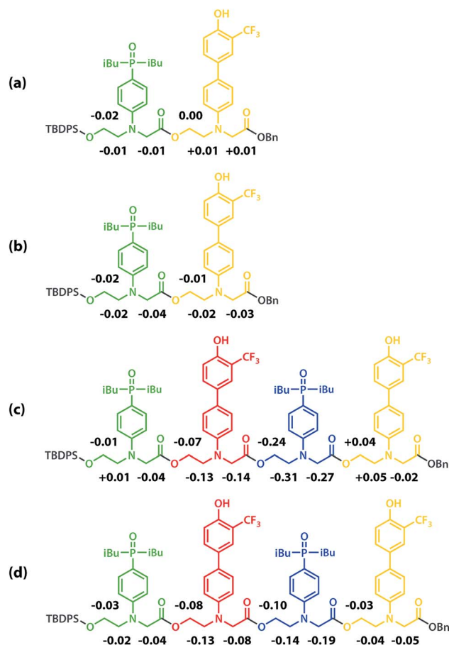
Fig. 9 Differences in the ^1\text{H} NMR chemical shifts ( \Delta\delta /ppm) of the signals due to the backbone protons of (a) monomeric AD, (b) dimeric AD, (c) monomeric ADAD, and (d) dimeric ADAD compared with the signals due to the corresponding protons in AA or DD in \text{CDCl}_3 at 298 K.
