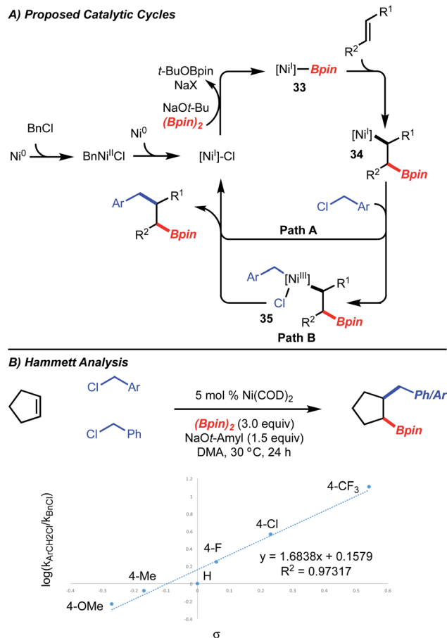
Scheme 5 Mechanistic studies.
