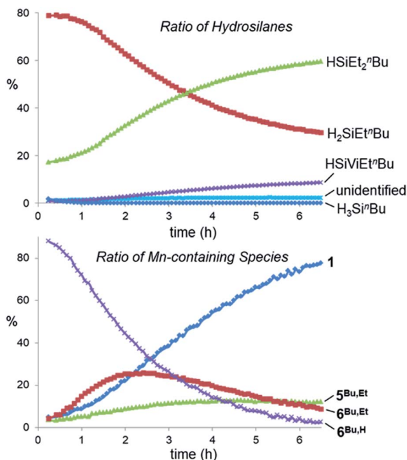
Fig. 10 Graphs showing the ratio of (top) hydrosilanes (dark blue ◆ = \text{H}_3\text{Si}^n\text{Bu} ; red ■ = \text{H}_2\text{SiEt}^n\text{Bu} ; green ▲ = \text{HSiEt}_2^n\text{Bu} ; purple × = \text{HSiViEt}^n\text{Bu} ; light blue * = unidentified \text{SiH} -containing silane) and (bottom) MnH-containing species {dark blue ◆ = [(\text{dmpe})_2\text{MnH}(\text{C}_2\text{H}_4)] (1); red ■ = [(\text{dmpe})_2\text{MnH}(\text{BuEtSi}=\text{CHMe})] ( 6^{\text{Bu,Et}} ); green ▲ = [(\text{dmpe})_2\text{MnH}_2(\text{SiHET}^n\text{Bu})] ( 5^{\text{Bu,Et}} ); purple × = [(\text{dmpe})_2\text{MnH}(\text{BuEtSi}=\text{CHMe})] ( 6^{\text{Bu,Et}} ) measured over time by ^1\text{H} NMR spectroscopy (in \text{C}_6\text{D}_6 at 56^\circ\text{C} ) for the hydrosilylation of ethylene (initial, n_{\text{C}_2\text{H}_4} \approx n_{\text{silane}} ) by a mixture of hydrosilanes corresponding to the 13 h mark in Fig. 9. Reaction details can be found in the ESI pg. S15.†
