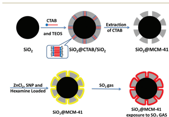
Scheme 1 Schematic illustration of the fabrication and detection processes of \text{SiO}_2@\text{MCM}-41 .
