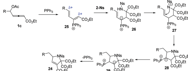
Scheme 8 Plausible mechanisms.
