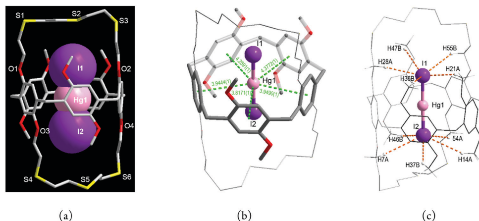
Fig. 4 The contact ion-triplet complex with mercury(II) iodide [(\text{I-Hg-I})@L] ( 3 ): (a) general view showing an ( \text{I}^- - \text{Hg}^{2+} - \text{I}^- ) entity (space-filling) in the central cavity, (b) a pentagonal bipyramidal geometry with five \text{Hg}^{2+}\cdots\pi interactions (green dashed lines) and an \text{I-Hg-I} axis and (c) a mercury-shared double pentagonal pyramidal geometry with five \text{C-H}\cdots\text{I}^- H-bonds (orange dashed lines) and \text{I-Hg-I} axis (only H-bonded H atoms are shown).
