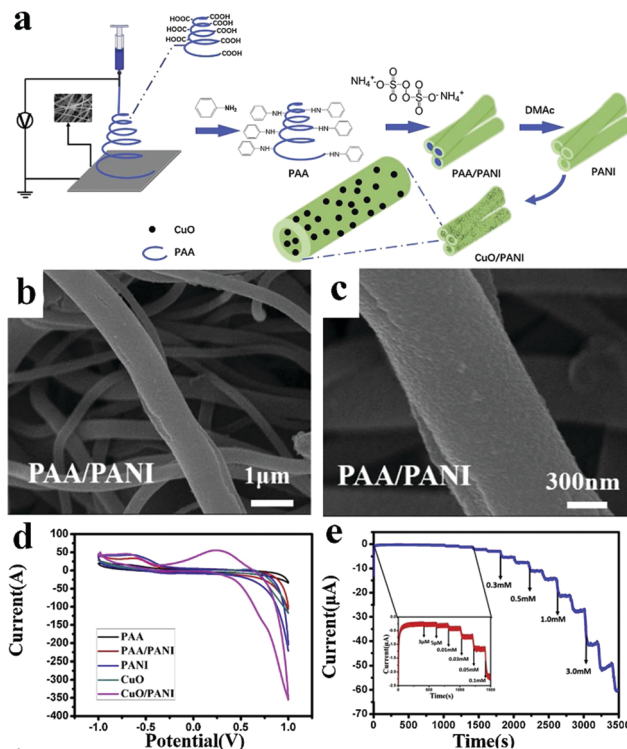
Fig. 6 (a) Schematic diagram of \text{CuO}/\text{PANI} nano-hybrid fiber synthesis. (b) Low magnification SEM image of the PAA hybrid nanofiber covered by PANI. (c) High magnification SEM image of the PAA hybrid nanofiber covered by PANI. (d) CV curves of GCEs modified with \text{CuO}/\text{PANI} nano-hybrid fibers. (e) Amperometric response of GCEs modified with \text{CuO}/\text{PANI} nano-hybrid fibers. Reproduced ref. 48 with permission from Elsevier B.V., copyright 2019.
