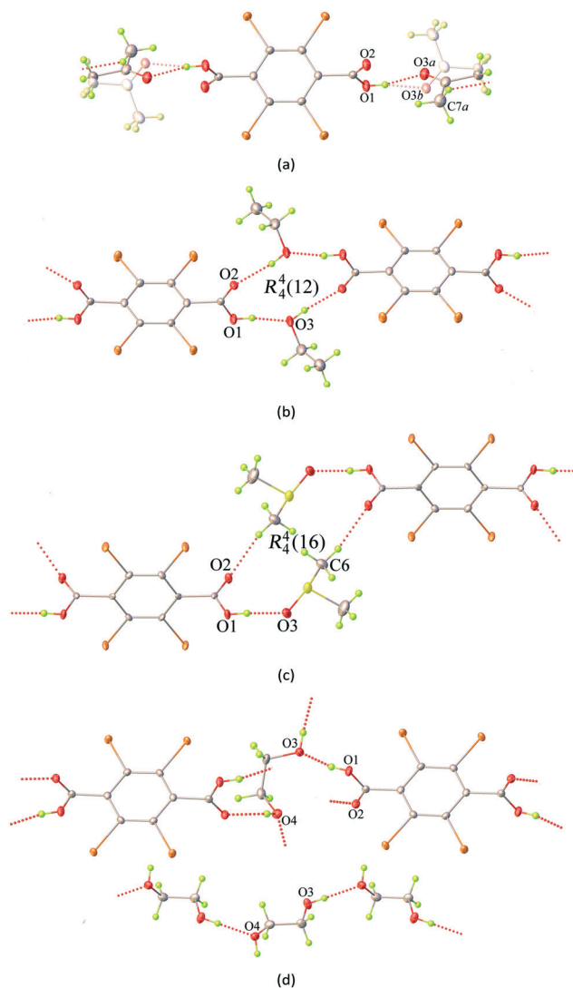
Fig. 2 Detail of the O/C–H \cdots O hydrogen bonding interactions (red dashed-lines) between the H 2 Br 4 BDC molecules and the solvents for the solvates (a) 1 ATN , (b) 2 EtOH , (c) 3 DMSO , and (d) 4 EG . The head-to-tail O–H \cdots O hydrogen bonding interactions between the EG molecules in 4 EG is also shown (d).
