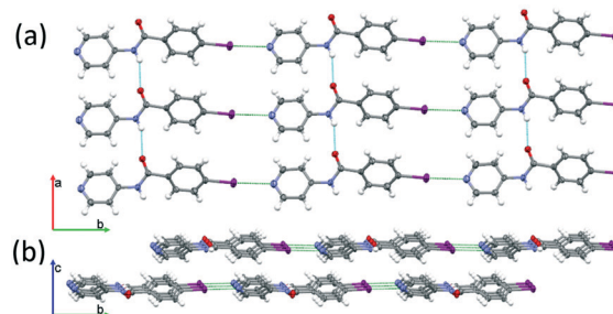
Fig. 3 INPBA structure: (a) 2D sheets formed by N_{\text{pyr}}\cdots I halogen bonding in green and perpendicular N-H\cdots O=C carboxamide hydrogen bonds in blue; (b) isolated layers. Thermal ellipsoids are drawn at the 50% probability level.
