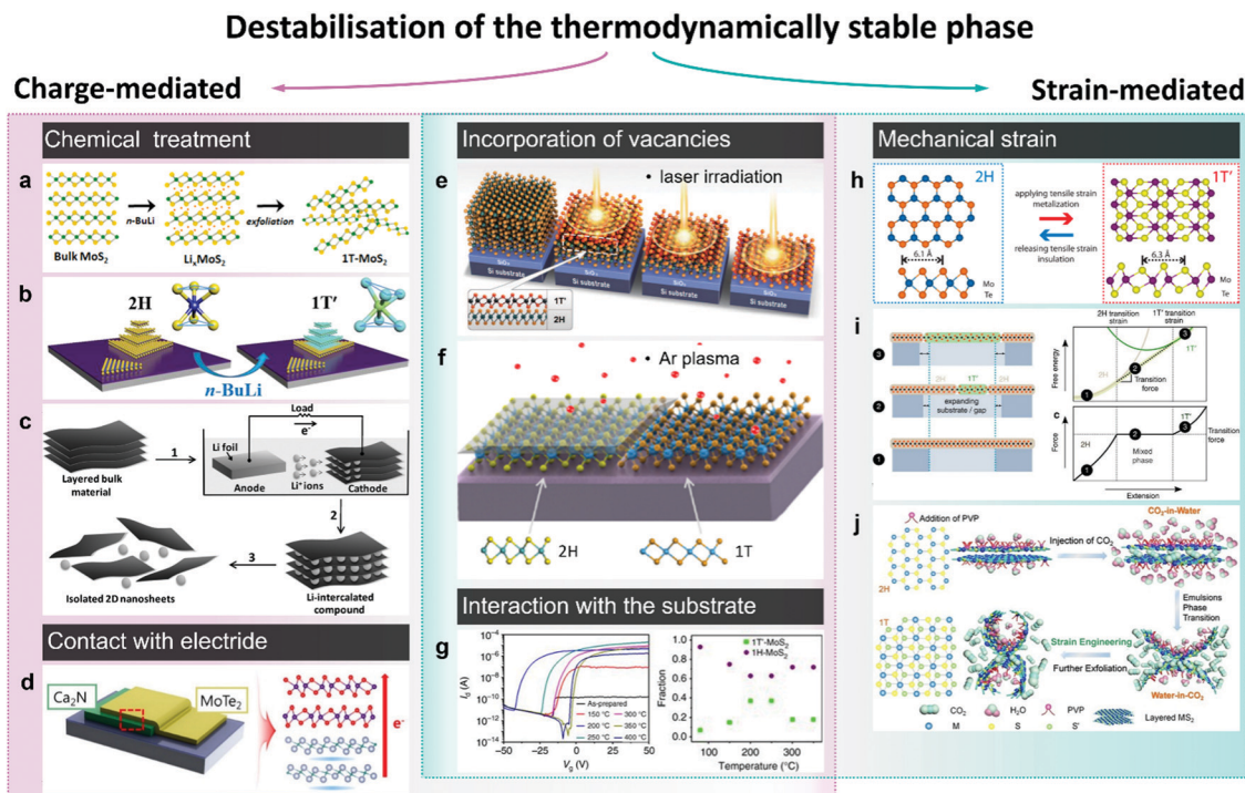
Fig. 3 Accessing the metastable 1\text{T}' phase via destabilisation of the thermodynamically stable ( 2\text{H} ) phase. The approaches to induce the 2\text{H} -to- 1\text{T}' transition in group VI TMDs are divided into two categories: charge-mediated, as chemical treatment (panels a–c) and contact with an electrode (panel d); and strain-mediated, such as tensile strain-induced transition between the 2\text{H} and 1\text{T}' ( 1\text{T} ) polymorphs (panels h–j). Panels e–g represent the phase transitions caused by the combination of charge and strain as in the case of chalcogen vacancies (panels e and f) or due to the interaction with the substrate (panel g). Separate panels are adapted with permission: (a) from ref. 100, copyright 2017, American Chemical Society; (b) from ref. 114, copyright 2018, American Chemical Society; (c) from ref. 108, copyright 2011, John Wiley & Sons; (d) from ref. 123, copyright 2017, American Chemical Society; (e) from ref. 155, copyright 2015, American Association for the Advancement of Science; (f) from ref. 138, copyright 2017, American Chemical Society; (g) from ref. 128, copyright 2017, Springer Nature; (h) from ref. 130, copyright 2016, American Chemical Society; (i) from ref. 25, copyright 2014, Springer Nature; and (j) from ref. 134, copyright 2017, John Wiley & Sons.
