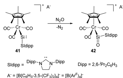
Scheme 19 Oxygenation of the metallocsilylene 41 with \text{N}_2\text{O} .
