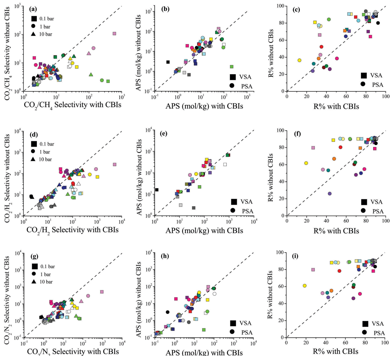
Fig. 5 Comparisons of the selectivity, APS, and R% values of MOFs with and without CBIs for separation of (a–c) \text{CO}_2/\text{CH}_4 : 50/50, (d–f) \text{CO}_2/\text{H}_2 : 15/85 and (g–i) \text{CO}_2/\text{N}_2 : 15/85 mixtures.
