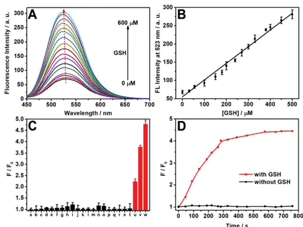
Fig. 1 (A) Fluorescence titration spectra of DTFN (0.3 mg mL -1 ) upon the addition of GSH (0–600 μM). (B) The linear relationship between the fluorescence intensity ( I_{523} ) and GSH (0–500 μM). (C) Fluorescence intensity ratio ( F/F_0 ) of DTFN upon exposure to various potential interferences, (a) blank (b) Na + (2 mM), (c) K + (2 mM), (d) Co 2+ (2 mM), (e) Ca 2+ (2 mM), (f) Mg 2+ (2 mM), (g) Ni 2+ (2 mM), (h) Cu 2+ (2 mM), (i) Fe 3+ (2 mM), (j) Ser (2 mM), (k) Asn (2 mM), (l) Thr (2 mM), (m) Gln (2 mM), (n) Gly (2 mM), (o) Ala (2 mM), (p) Arg (2 mM), (q) His (2 mM), (r) Met (2 mM), (s) BSA (1 mg mL -1 ), (t) glucose (2 mM), (u) GSH (200 μM), (v) GSH (400 μM), (w) GSH (600 μM). (D) Time-dependent fluorescent intensity ratio ( F/F_0 ) of DTFN in the absence of GSH (black) and in the presence of GSH (600 μM) (red). Note: F_0 and F are the fluorescence intensity of DTFN without and with addition of GSH, respectively.
