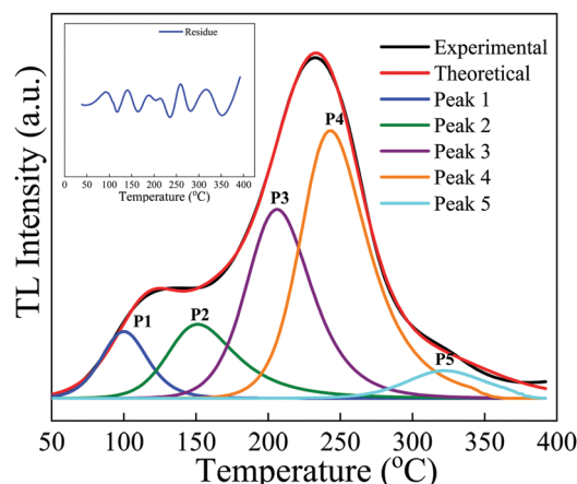
Fig. 13 The deconvoluted glow curves of the NaGdF 4 :3% Tb 3+ phosphor recorded after irradiation with a dose of 10 kGy gamma rays using the GCD program.
