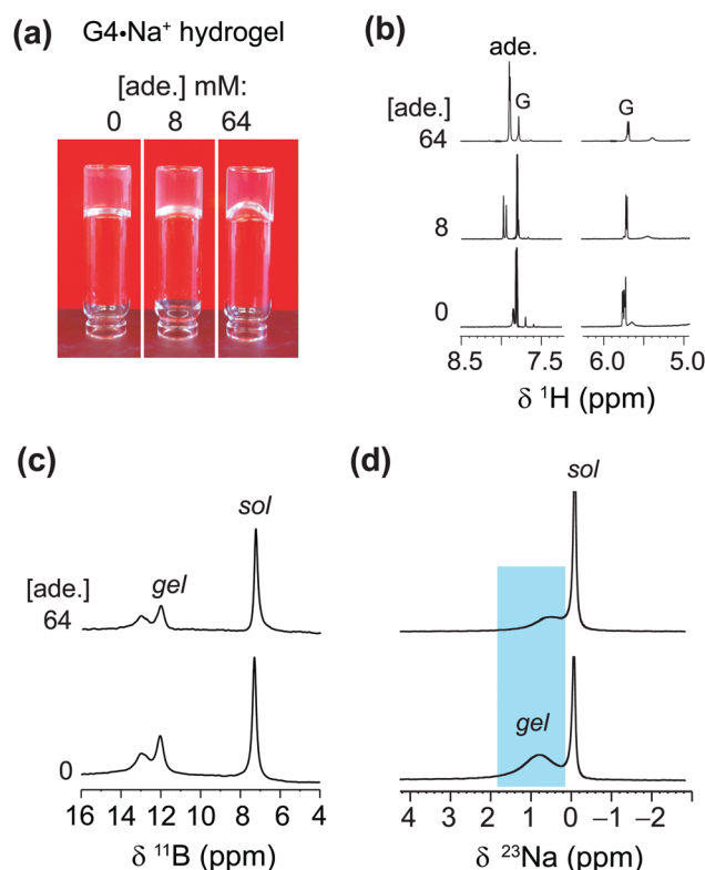
Fig. 5 (a) Photographs of 72 mM \text{G4-Na}^+ borate hydrogels taken before and after the incorporation of 8 mM and 64 mM of adenine. (b) ^1\text{H} (9.4 T, 400 MHz), (c) ^{11}\text{B} (20 T, 5 kHz MAS) and (d) ^{23}\text{Na} (20 T, 5 kHz MAS) NMR spectra of \text{G4-Na}^+ borate gels shown in the inverted vials in (a). Sol and gel signals correspond to free cations or molecules in a solution-like environment and in the G4 network, respectively.
