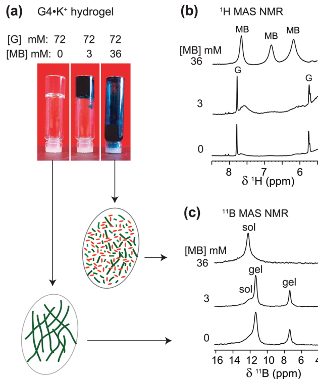
Fig. 3 (a) Photographs of 72 mM G4-M + borate hydrogels taken before and after the incorporation of 3 mM and 36 mM of MB, accompanied by 1D (b) 1 H and (c) 11 B (20 T, 5 kHz MAS) NMR spectra of G4-K + borate gels shown in the vials (similar 11 B MAS NMR spectra acquired at 11.7 T are presented in ref. 21). Inset figures in ovals represent schematics of G4 fibrils before and after the addition of methylene blue. Sol and gel 11 B signals correspond to borate mono- and diesters in a solution-like environment and in the G4 network, respectively.
