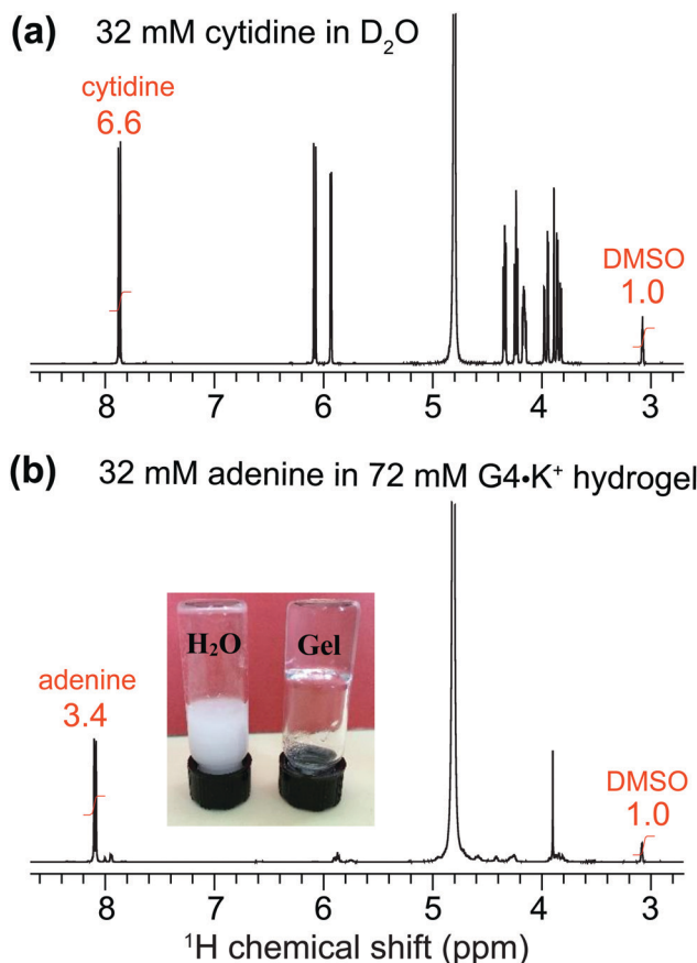
Fig. 4 Solution-state 1D ^1\text{H} (600 MHz) NMR spectrum of (a) 32 mM of cytidine dissolved in D 2 O using DMSO proton signals (at 3.09 ppm, integral of 1.0) as an internal calibration standard, and (b) of 32 mM adenine incorporated into a G4-K + gel. The inset image in (b) depicts the dissolution of 32 mM of adenine in H 2 O (left) and in 72 mM G4-K + borate gel (right).
