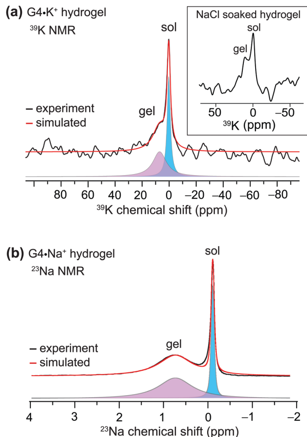
Fig. 1 Gel-state 1D MAS NMR spectra of 20 \mu\text{L} \text{G4}\cdot\text{M}^+ hydrogels acquired at 20 T with their deconvolution into broad and narrow components: (a) ^{39}\text{K} MAS (5 kHz) NMR spectrum of \text{G4}\cdot\text{K}^+ gel and (b) ^{23}\text{Na} MAS (5 kHz) NMR spectrum of \text{G4}\cdot\text{Na}^+ gel. The inset in (a) depicts a ^{39}\text{K} MAS NMR spectrum of a \text{G4}\cdot\text{K}^+ borate gel that had been soaked overnight in 155 mM NaCl solution, acquired under the same conditions. The narrow and broad signals originate from the free cations in the solution-like environment (herein called sol) and cations associated with the G4 network (herein called gel), respectively.
