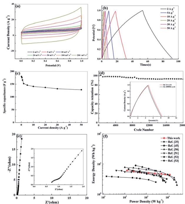
Fig. 8 Electrochemical performances of N, O-PC-CNTs symmetric supercapacitor devices using 6 \text{ mol L}^{-1} KOH as electrolyte, (a) CV profiles at various scan rates in a potential range of 0–1 V, (b) GCD curves at different current densities, (c) specific capacitance of N, O-PC-CNTs at different current densities, (d) cycling stability of the devices at 20 \text{ A g}^{-1} , (e) Nyquist plots, and (f) Ragone plots.
