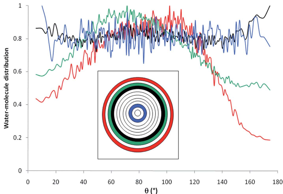
Fig. 6 Water molecules orientations inside the nanopore (filled with pure water); \theta represents the angle composed by the water dipole moment and the normal vector. The inset shows the location of the different layers inside the pore ( n = 12 ).
