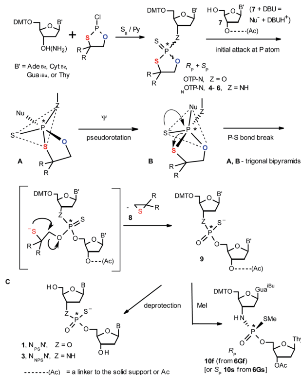
Scheme 1 A mechanism of the DBU-promoted condensation step in Otp synthesis of N_{PS}N' or N_{NPS}N' with the use of a mixture of P-epimers of OTP-N ( Z = O ) or N_{OTP}-N ( Z = NH ), respectively. 4 , R = H ; 5 , R = Me ; 6 , R, R = -(CH_2)_5- . B' = Ade^{Bz} , Cyt^{Bz} , Gua^{iBu} , or Thy . The codes 6Gf and 6Gs indicate fast- and slow-eluting P-diastereomers of Pm-N_{OTP}-dG ( vide infra ).
