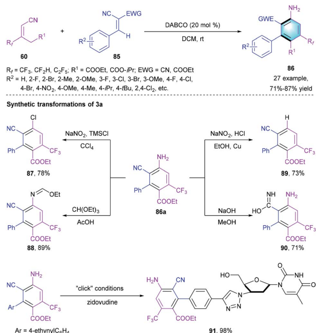
Scheme 25 DABCO-catalyzed [4 + 2] benzannulation to synthesize biaryls.
