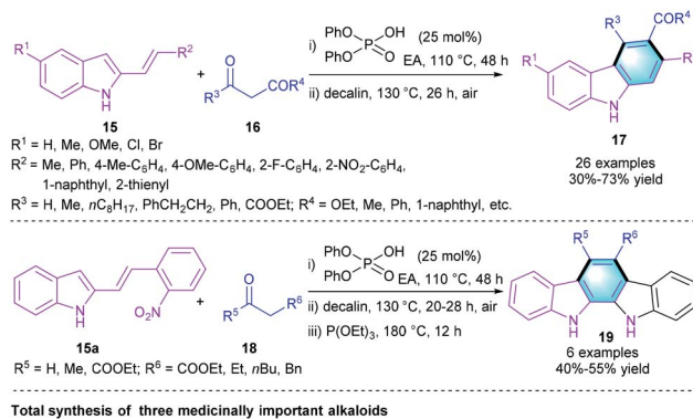
Scheme 4 Phosphoric acid-catalyzed [4 + 2] benzannulation to synthesize carbazoles and indolocarbazoles.
