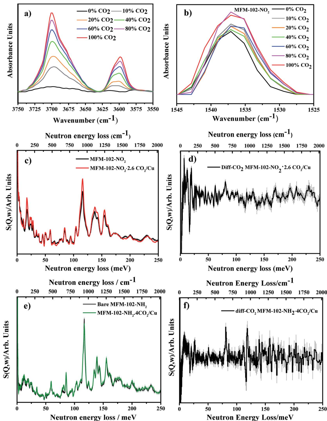
Fig. 5 (a) IR spectra showing the adsorption of \text{CO}_2 into MFM-102- \text{NO}_2 and demonstrating the growth in \nu_1 + \nu_3 and 2\nu_2 + \nu_3 combination bands for \text{CO}_2 near 3700 \text{ cm}^{-1} and 3600 \text{ cm}^{-1} . (b) Changes in intensity and broadening of the \text{N}=\text{O} asymmetric stretching vibration with \text{CO}_2 loading. (c) INS spectra for activated MFM-102- \text{NO}_2 and MFM-102- \text{NO}_2 with \text{CO}_2 loading. (d) Difference INS plot, derived by subtracting INS spectra for \text{CO}_2 -loaded MFM-102- \text{NO}_2 and bare MFM-102- \text{NO}_2 spectra. (e) and (f) are the same as (c) and (d), respectively, but replacing MFM-102- \text{NO}_2 with MFM-102- \text{NH}_2 .
