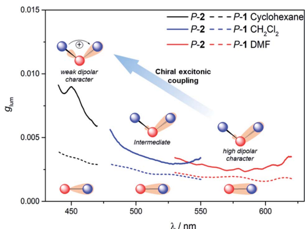
Fig. 5 Emission dissymmetry factors g_{\text{lum}} of P -1 (dashed lines) and P -2 (solid lines) in cyclohexane (black), \text{CH}_2\text{Cl}_2 (blue), and DMF (red) at 298 K ( \sim 10^{-5} M) along with illustration of the effects underlying the observed trends.
