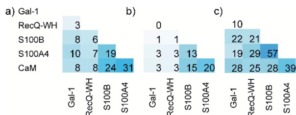
Fig. 7 Pairwise scaled covariances (%; maximum similarity: 100%, zero covariance: 0%) of H14 LSM F_B patterns calculated for total (a) and the orthosteric (b) F_B values. The sequence homologies of proteins are given in panel (c).
