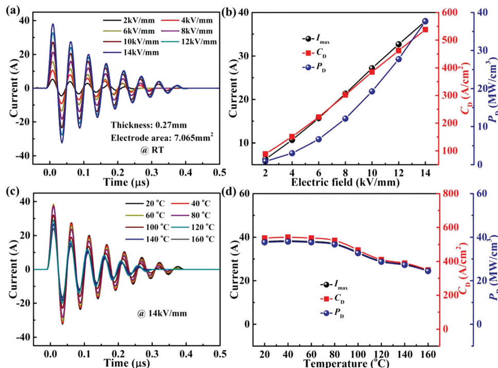
Fig. 9 (a) Underdamped discharge waveforms of the 0.22BMT ceramics under various electric fields and room temperature. (b) Variations of I_{\text{max}} , C_D , and P_D as functions of the applied electric field. (c) Underdamped discharge waveforms of the 0.22BMT ceramics at different temperatures under 14 kV mm -1 . (d) Variations of I_{\text{max}} , C_D , and P_D as functions of the temperature.
