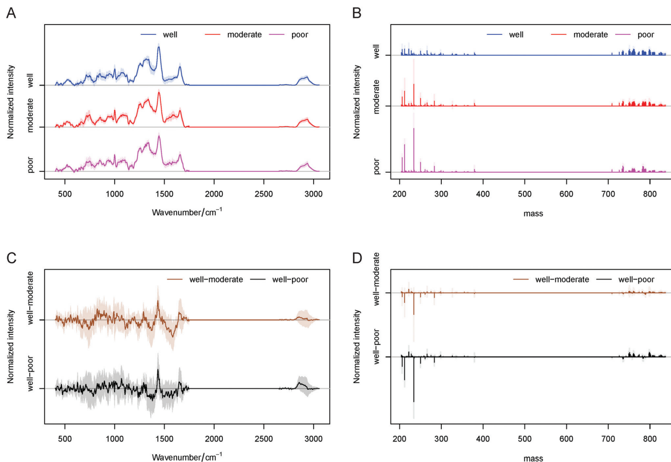
Fig. 5 Raman spectra (A) and MALDI spectra (B) of the three differentiation grades of liver cancer. The average spectra and their standard deviations are shown for well-, moderately- and poorly-differentiated HCC. Difference spectra between the spectra of the different grades are calculated for both measurement methods and they are shown in (C) and (D).
