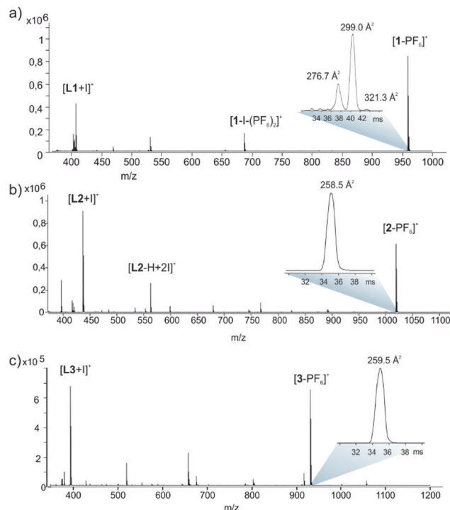
Fig. 3 (+)ESI-QTOF mass spectrum (a) 1 , (b) 2 and (c) 3 in MeCN. Insets show IM-TOF arrival time distributions for ions [C-PF_6]^+ .
