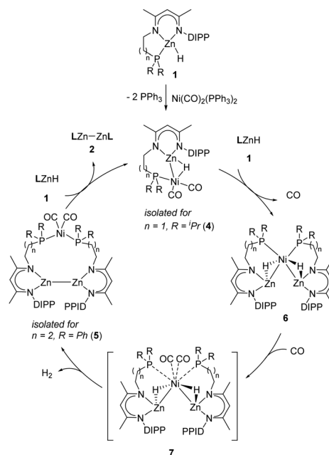
Scheme 3 Plausible mechanistic framework for Ni-catalyzed synthesis of Zn–Zn bonded compounds.
