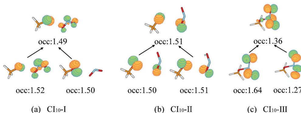
Fig. 4 The natural transition orbitals along with their fractional occupation numbers at the S_1 \rightarrow S_0 MECIs optimized at the SA(4)-CASSCF(12,9)/cc-pVDZ level.
