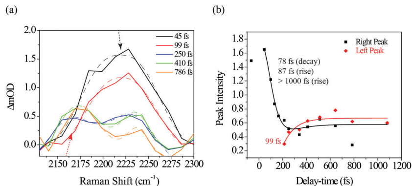
Fig. 7 (a) Closeup of the Raman shift region around 2100–2300 \text{cm}^{-1} where the ODIBO \text{S}^1_{\text{C}\equiv\text{C}} feature is expected. The spectra at the different time-delays are fit with single and double Gaussians (dotted lines) to describe the peak's change from a single to double-peak feature at \sim 200 fs delay time. (b) Intensity dynamics of the left ( 2165 \text{ cm}^{-1} ) band and right ( 2230 \text{ cm}^{-1} ) band fit with a single and three-component exponential model, respectively (solid curves).
