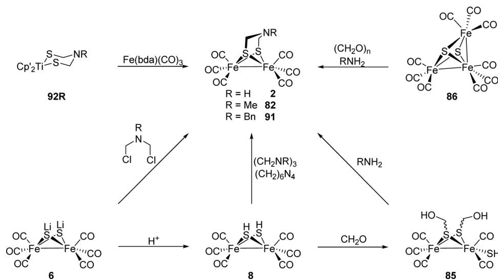
Fig. 31 Synthetic pathways towards \text{Fe}_2(\text{adt}^{\text{R}})(\text{CO})_6 mimics. (Cp' = MeC 5 H 4 ).
