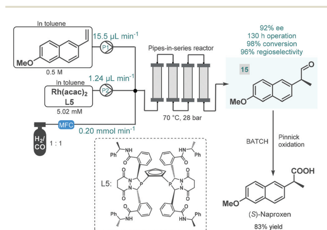
Scheme 6 Continuous flow enantioselective synthesis of a chiral naproxen precursor. 62
